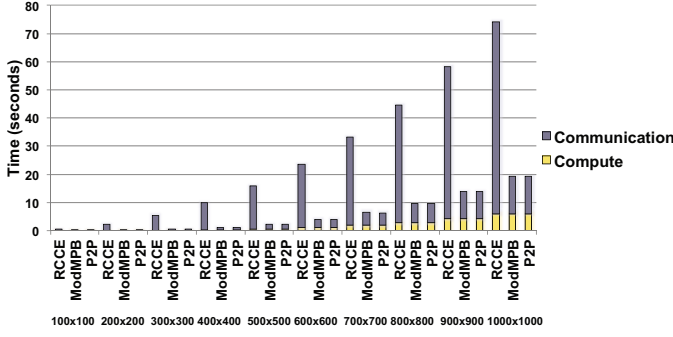
Fig. 14. Matrix multiply execution time broken down into time spent on compute and communication for various input matrix sizes.
