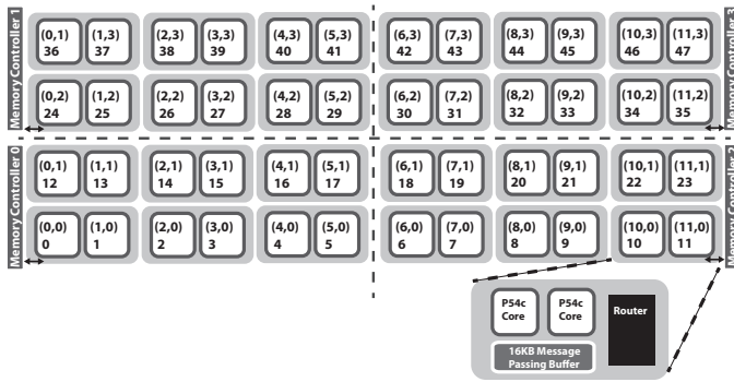
Fig. 1. Intel SCC Tile Layout.
