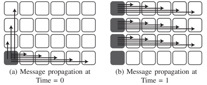
Fig. 7. ModMPB Broadcast Propagation.
