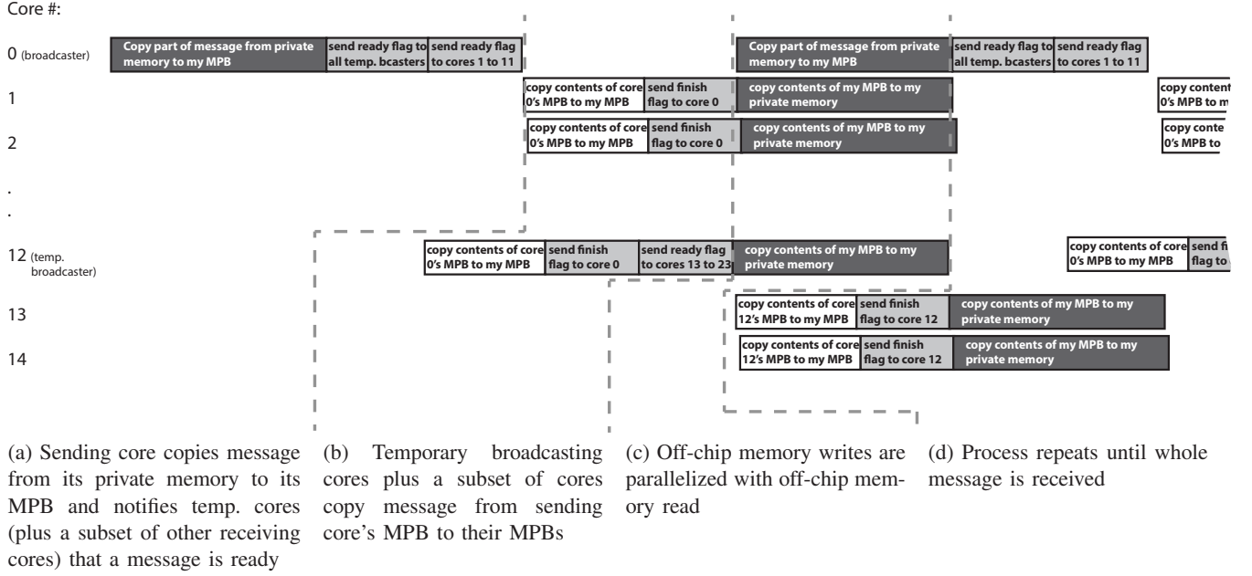
Fig. 8. ModMPB Broadcast Timing Diagram
