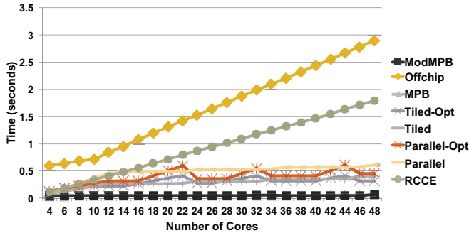
Fig. 11. Microbenchmark results: Broadcast latency when varying number of participating cores.
