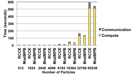
Fig. 15. N-Body execution time broken down into time spent on compute and communication for varying numbers of particles (each particle is 32 bytes).
