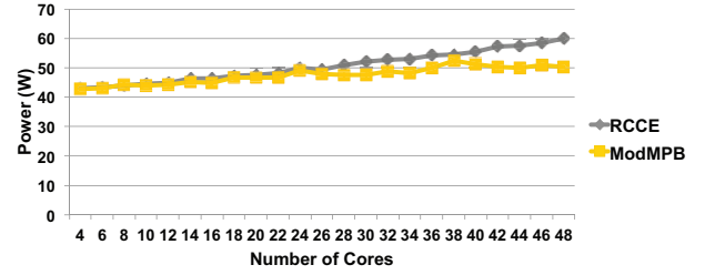
Fig. 17. Power consumption for RCCE and ModMPB broadcasts.
