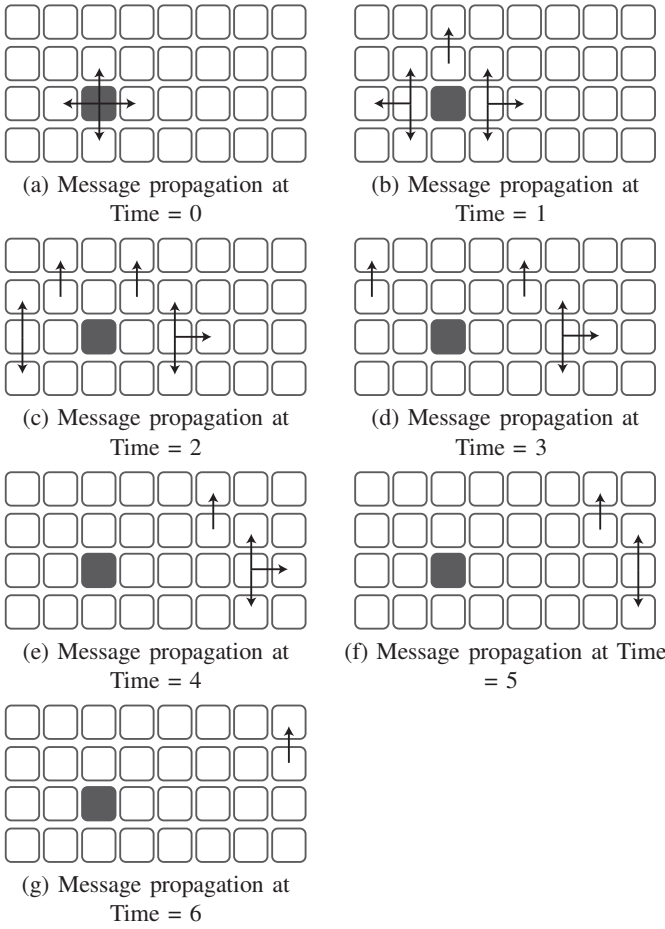
Fig. 2. Parallel Broadcast Propagation. The broadcast source node is shown in grey. The number of cores shown is simply for illustration purposes.
