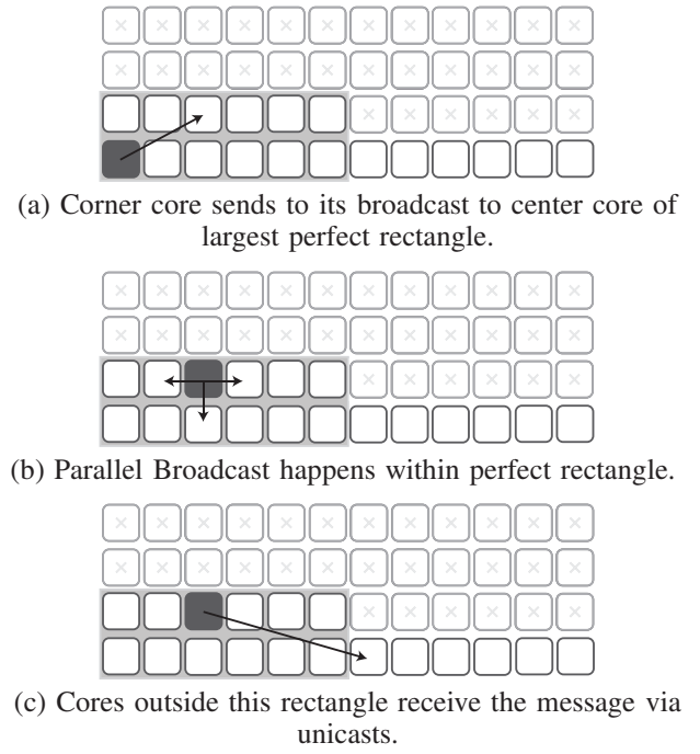
Fig. 12. Optimized Parallel Broadcast with 18 active cores. The maximum perfect rectangle is shown in light grey. Cores not participating in the broadcast are marked with a “x”.
