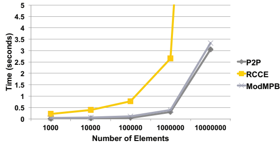
Fig. 16. Bucket sort communication latency (comparing bucket sort algorithms that use broadcasts to an algorithm that uses only point-to-point communication).
