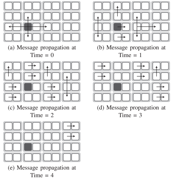
Fig. 4. Tiled Parallel Broadcast Propagation. Tiles are shown in grey. Once one core in a tile receives the broadcast, it first forwards the message to the adjacent tile and then sends the message to the adjacent core within its own tile.
