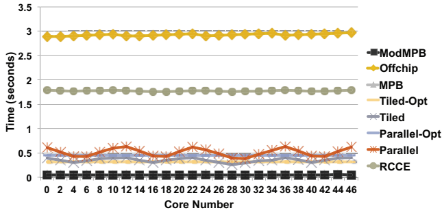
Fig. 10. Microbenchmark results: Broadcast latency when varying broadcasting source core.
