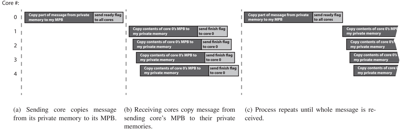
Fig. 6. MPB Broadcast Timing Diagram.
