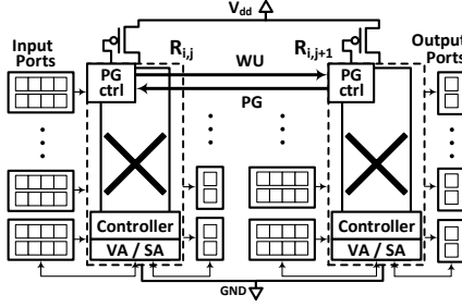
Fig. 1: Power Gating of On-Chip Routers.
