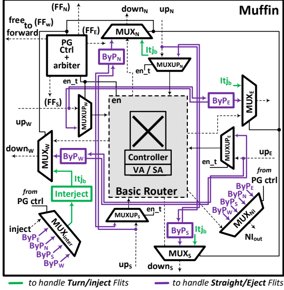
Fig. 2: Muffin Router Micro-Architecture.
