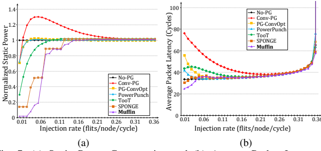
Fig. 7: (a) Static Power Consumption and (b) Average Packet Latency, in Uniform Synthetic Traffic.
