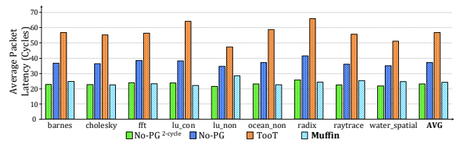
Fig. 9: Average Packet Latency using Adaptive Routing.
