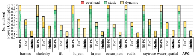
Fig. 8: Power Breakdown using Adaptive Routing.
