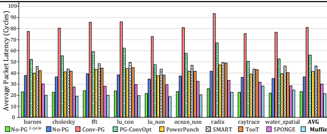
Fig. 5: Average Packet Latency.
