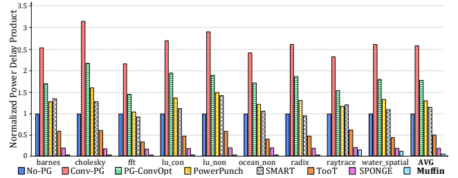
Fig. 6: Normalized Power Delay Product.
