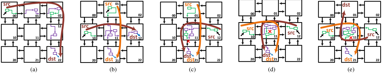
Fig. 3: Example flow control in Muffin when basic routers are power gated (a) Single Flit and No Contention, (b) Multi Flit and No Conflict, (c) Contention of Straight and Turn , (d) Contention of two Turns on Same Downstream Link, (e) Contention of two Turns on Different Downstream Links.
